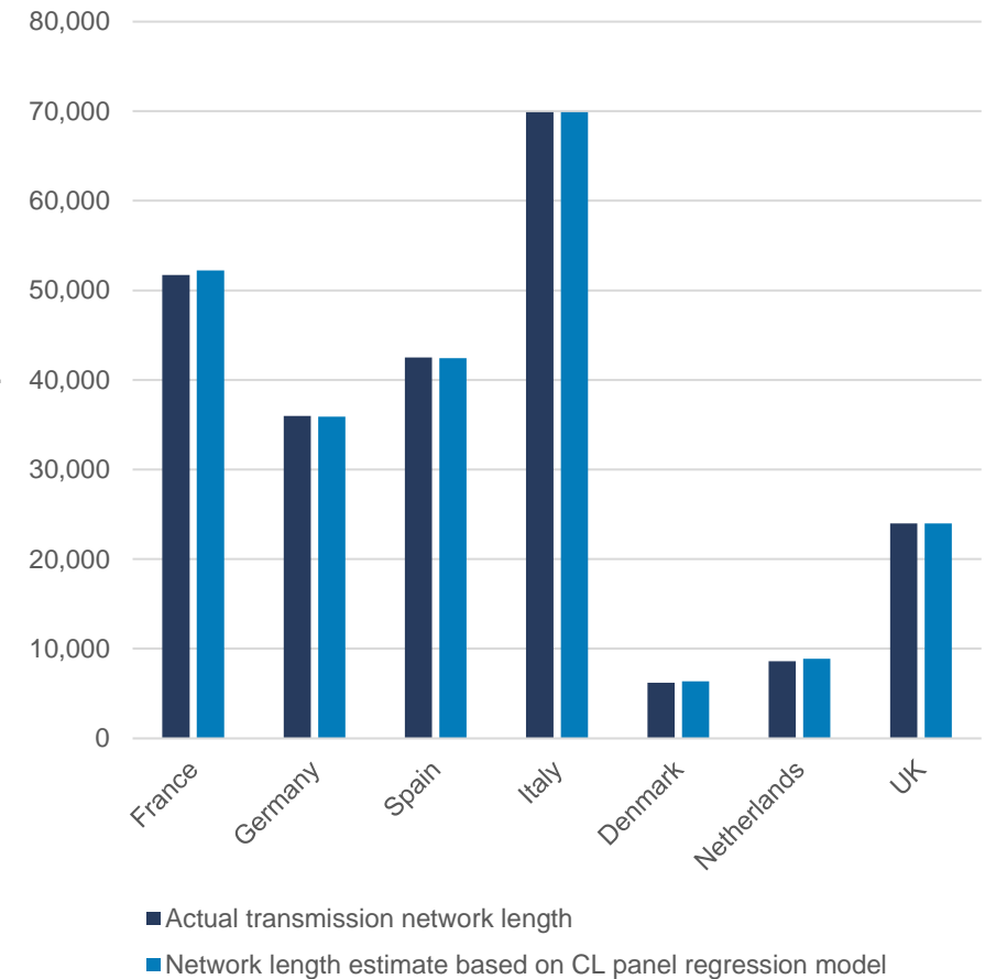
Panel regression model – Estimated vs. actual length of transmission network length in 2022 (km)
