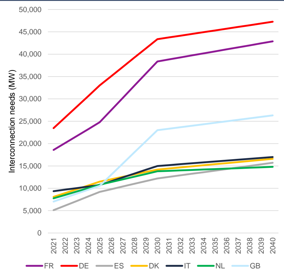
Interconnection needs (MW) – ENTSO-E IoSN TYNDP 2022
