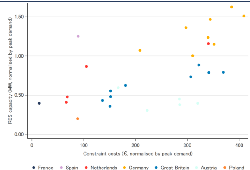
Relationship between RES capacity and congestion costs > 1 m€ (normalised by peak demand), 2015-2022
